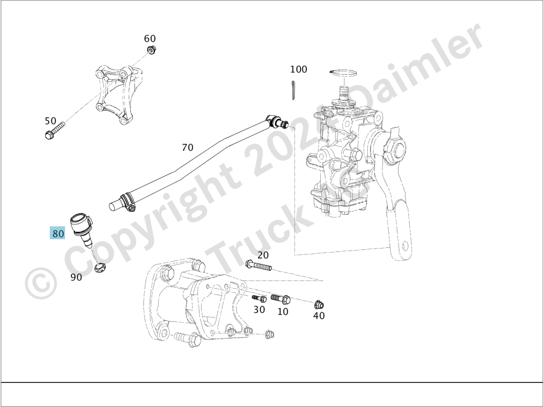
Image ID: drawing_PV000.003.027.979_version_001
